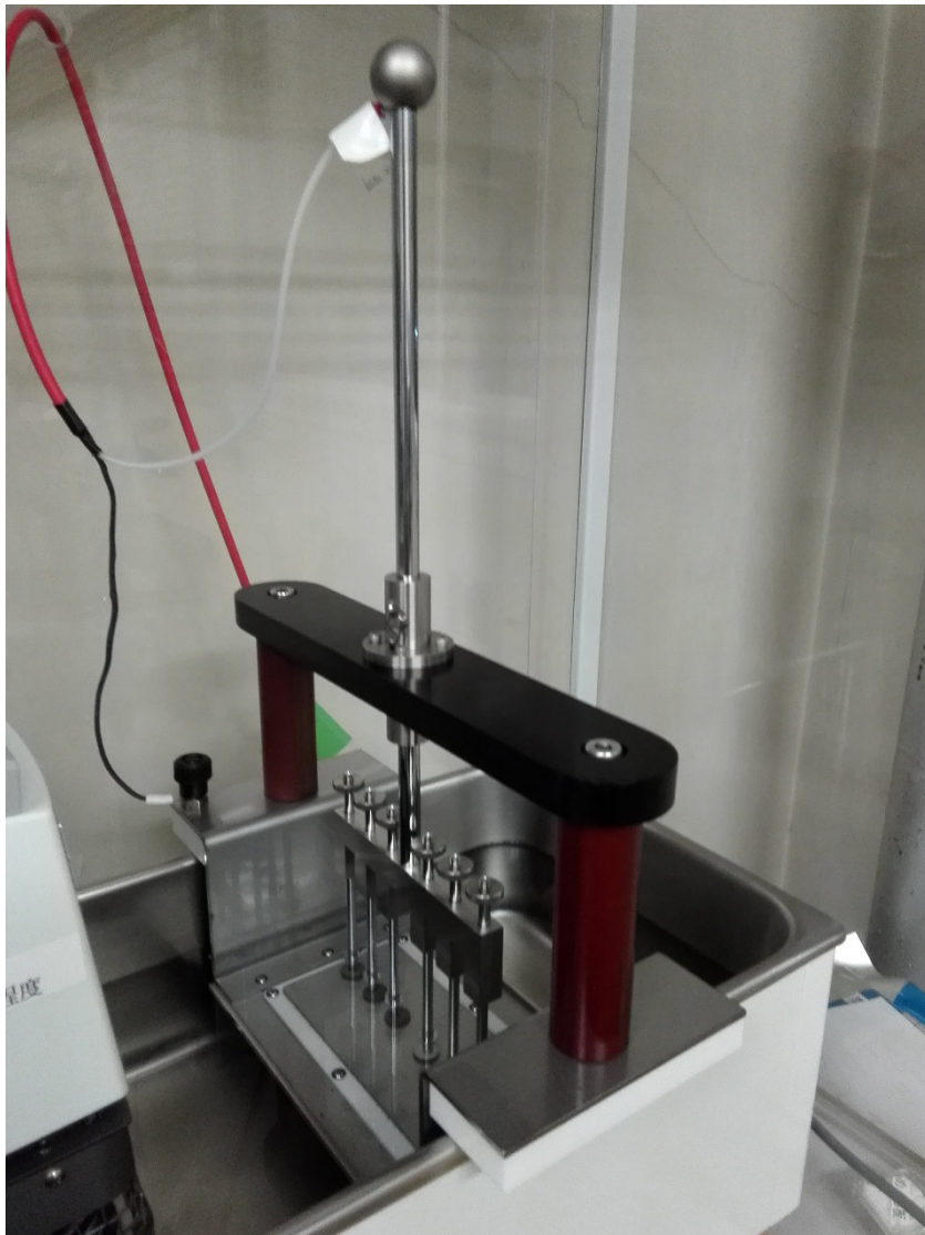
polarizing apparatus 10kVmax, 150degreesCmax
