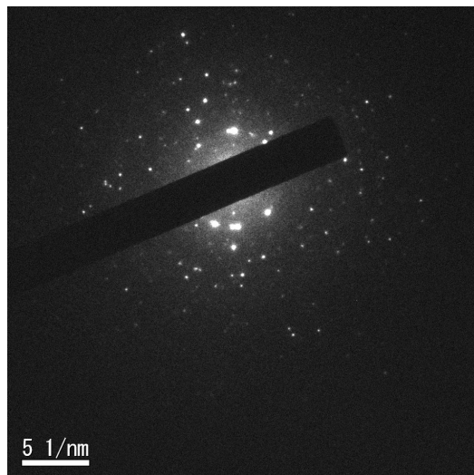
Diffraction pattern of many single crystal nanocubes
